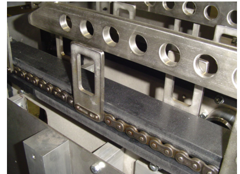
Standard sized lugs, carrier chains and chain track rails are all available in stock
